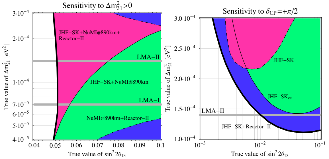
Figure 7: Synergies from the combination of JHF-SK, NuMI (at 890 km) and a Reactor-II experiment. The left plot shows the parameter space in the \Delta m_{31}^2 - \sin^2 2\theta_{13} plane where \text{sign}(\Delta m_{31}^2) can be determined. It can be seen that the combination is sensitive to \text{sign}(\Delta m_{31}^2) independently of \Delta m_{31}^2 for \sin^2 2\theta_{13} > 0.05 . The right plot shows the parameter space in the \Delta m_{31}^2 - \sin^2 2\theta_{13} plane where a CP phase \delta = \pi/2 could be determined. The improvement comes here mostly from the fact that the reactor measurement allows the beams to run fully with neutrinos. For details see 34) .
