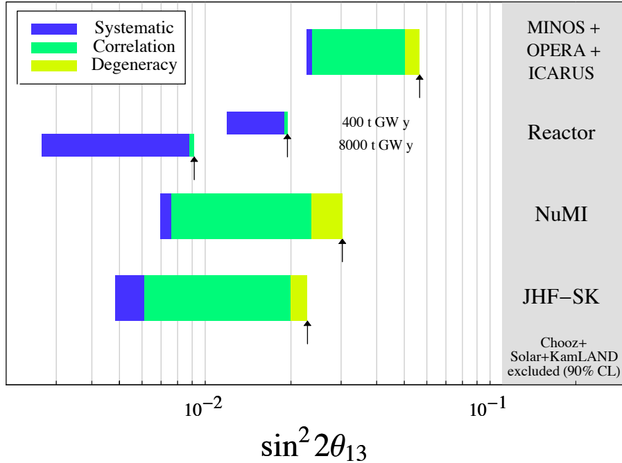
Figure 6: The \theta_{13} sensitivity of potential reactor experiments compared to accelerator experiments which could be built on similar time scales. MINOS+OPERA+ICARUS is what can be obtained from the combination of these experiments. The results for the scenarios Reactor-I and Reactor-II are significantly better and they cut into the correlation and degeneracy range of NuMI and JHF-SK. This shows that there is synergy between a new reactor experiment and JHF-SK and NuMI. See figure 3 for the colour coding.
