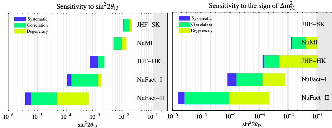
Figure 3: Left plot: The \theta_{13} sensitivity of different future accelerator based neutrino oscillation experiments 20 ). Right plot: The \theta_{13} values for which sensitivity to matter effects, i.e. sign(\Delta m^2_{31}) exists. The shown bands are again the reduction of sensitivity from a purely statistical limit (left end of the dark grey/blue range) by systematics (right end of dark grey/blue), correlations (medium grey/green) and degeneracies (light grey/yellow). The right end of the light grey (yellow) band represents the final 90%CL limit. The grey area for large \sin^2 2\theta_{13} indicates the current limit from the Chooz experiment.
