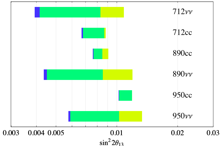
Figure 4: The \theta_{13} sensitivity of different combinations of the JHF-SuperKamiokande and NuMI off-axis experiments. The labels indicate for different scenarios the NuMI baseline in km and the type of beam for JHF-SK (first character) and NuMI (second character). \nu stands for neutrino beams only, while c stands for combined neutrino and anti-neutrino running. The color coding is as defined in the caption of fig. 3 and the right edge of the bars corresponds to the sensitivity limit of each setup 18) .
