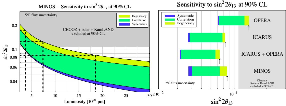
Figure 2: Left plot: The sensitivity of the MINOS experiment to \theta_{13} as a function of the protons on target (pot) assuming a 5% flux uncertainty. The grey (colored) bands show the reduction of sensitivity from a purely statistical limit (lower end of the dark grey/blue band) by systematics (dark grey/blue), correlations (medium grey/green) and degeneracies (light grey/yellow). The upper end of the light grey (yellow) band represents the final 90%CL limit. The dashed lines represent what 1, 2 and 5 years of operation might achieve (from left to right). Right plot: Comparison of 5 years of operation for the MINOS and CNGS experiments. The grey area for large \sin^2 2\theta_{13} indicates in all cases the current limit from the Chooz experiment. Further details can be found in a forthcoming paper 32 ).
