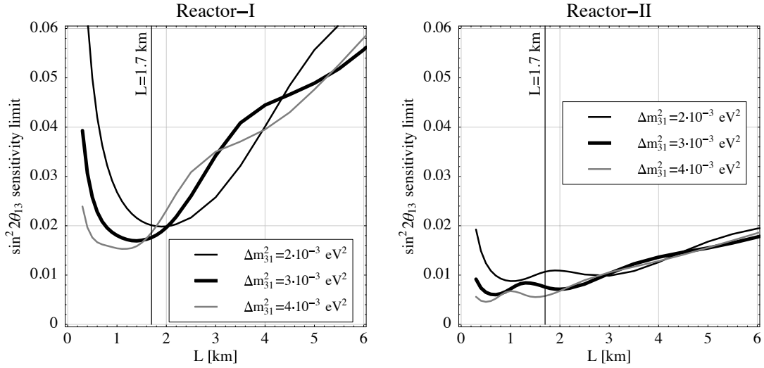
Figure 5: The \sin^2 2\theta_{13} sensitivity of reactor experiments as a function of the distance of the far detector. Shown are two scenarios. Reactor-I assumes for the product of detector mass, reactor thermal power and running time 400t GW y. Reactor-II corresponds to 8000t GW y. Reactor-I could, for example, be realized by a 10t detector, 8GW thermal power and 5 years of data taking 34) .
