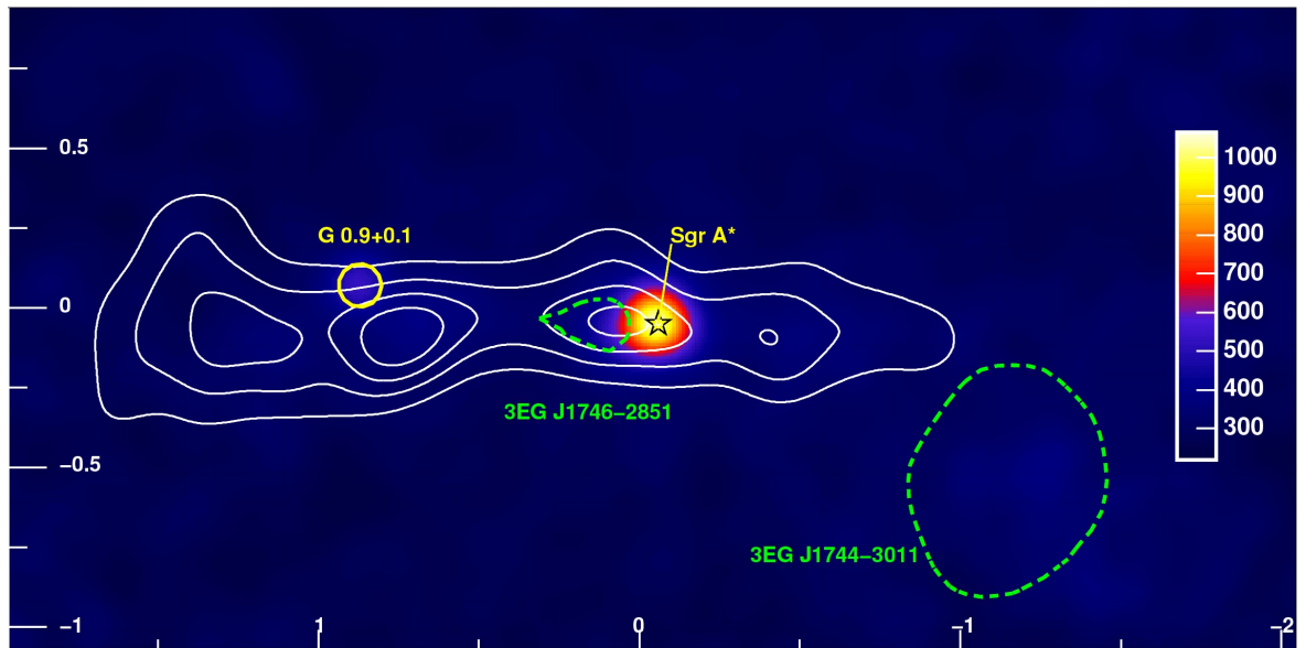
Figure 1. Smoothed and acceptance corrected count map of the Galactic Centre region from H.E.S.S. observations in 2004. The known VHE \gamma -ray sources G 0.9+0.1 and HESS J1745–290 (coincident with Sgr A * ) are marked with a circle and a star, respectively. The 90% confidence contours are given for the positions of the two unidentified EGRET sources in this region (green dashed lines). The solid contours show CS emission smoothed to match the H.E.S.S. point spread function.
