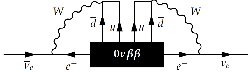
Figure 1.2: Schechter-Valle or black box theorem. Figure taken from [122].
