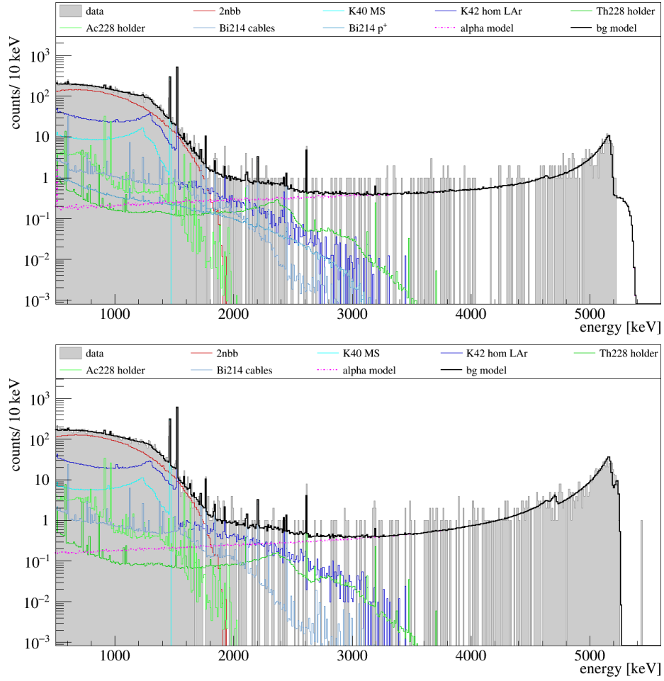
Figure 8.2: Energy spectra of the first six month of Phase II data with preliminary background model. Top: BEGe dataset. Bottom: Semi-coaxial dataset.
