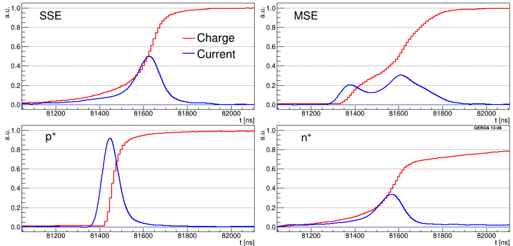
Figure 2.5: Characteristic charge and current signals of single site events (SSE), multi site events (MSE), events on the p^+ surface and on the n^+ surface in a BEGe detector. The figure has been taken from [17].
