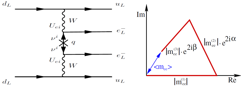
Figure 1.3: Left: quark level ‘lobster’ diagram for neutrinoless double-beta decay in case of light Majorana neutrino exchange. Right: geometrical visualization of the effective mass ( \alpha , \beta are defined as \alpha = 2\alpha_1 and \beta = \alpha_2 - \delta_{CP} with \alpha_1 , \alpha_2 and \delta_{CP} the phases from the U_{PMNS} matrix. Figure taken from [121].
