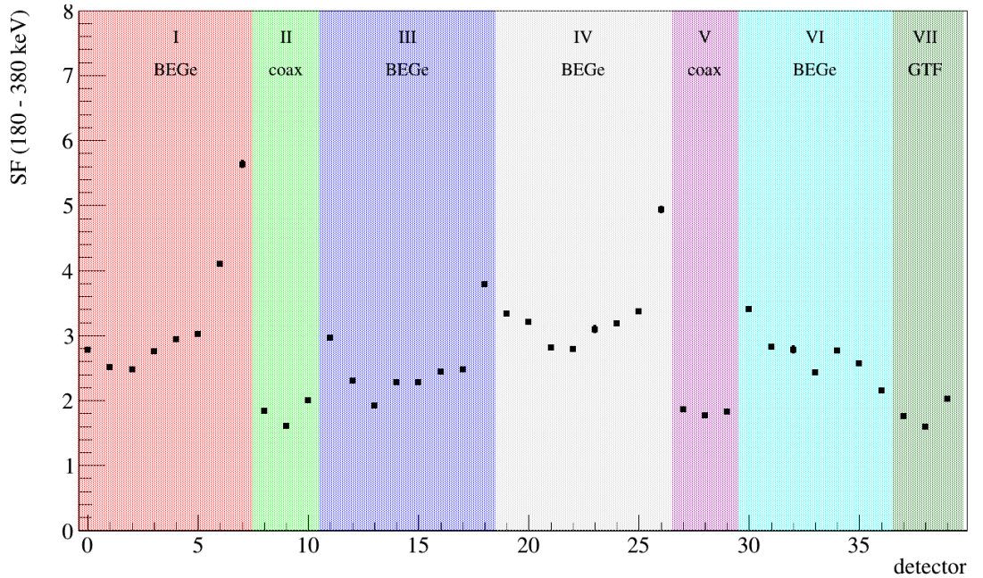
Figure 7.20: ^{39}\text{Ar} suppression by the LAr veto for the individual Germanium detectors.
