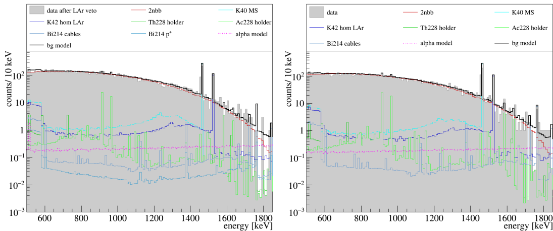
Figure 8.5: Energy spectra after LAr veto with an approximative background model. Left: BEGe dataset. Right: Semi-coaxial dataset.
