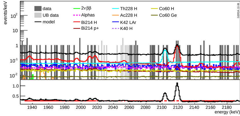
Figure 2.8: Measured energy spectrum and background model. In the upper part the measured counts in the ROI are shown in gray. Superimposed are the full background model (black) along with the fitted individual background sources (colored). Contaminations in the detector holders are denoted H , contaminations in the Germanium detector volume Ge , radioactive background sources in the LAr close to the detectors are labeled LAr and background sources close to the readout electrodes are denoted p^+ . At the bottom, the background spectrum obtained from the background model (black) has been fitted with a constant (red) representing a flat background.
