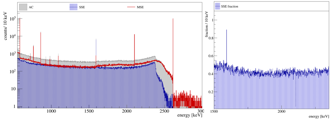
Figure 7.13: SSE and MSE contributions to ^{228}\text{Th} spectrum.
