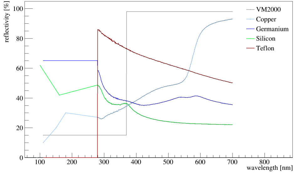
Figure 5.4: Reflectivities of materials as implemented in MaGe.
