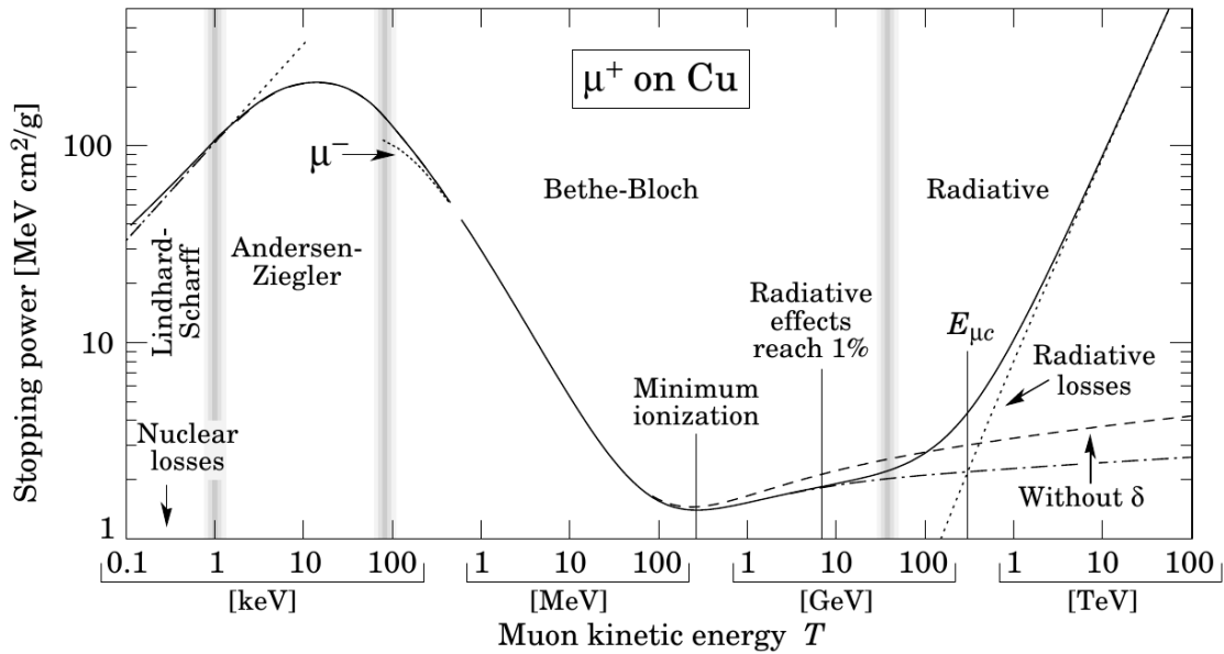
Figure 3.3: Muon stopping power for different energies in a moderately heavy material [Ber12].
