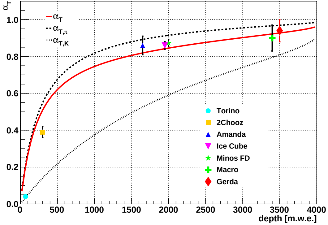
Figure 6.14: Correlation coefficient \alpha_T as a function of depth. Experiments are listed with different m.w.e. of rock overburden, such as Torino [Cas67], DOUBLE CHOOZ [Die13], AMANDA [Bou99], ICECUBE [Des11], MINOS far detector [Ada10], MACRO [Amb03] and GERDA (this work). GERDA and MACRO are located at the same depth but are drawn slightly apart for optical reasons. The dashed curves show muon generation models based on either purely pionic or only kaonic processes. The red line notes the literature value for the atmospheric kaon/pion ratio [Bar06].
