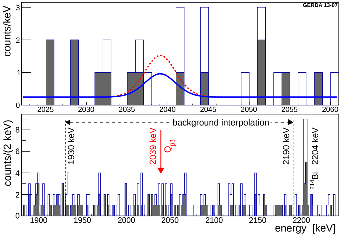
Figure 4.6: The combined energy spectrum of all ^{enr}\text{Ge} detectors is shown without (all) and with (grey) PSD. On the top, the region of interest around Q_{\beta\beta} is shown with the 90% upper limit derived from the data (blue line) and the central value from [KK04] (red dashes). On the bottom, the region for background interpolation is shown.
