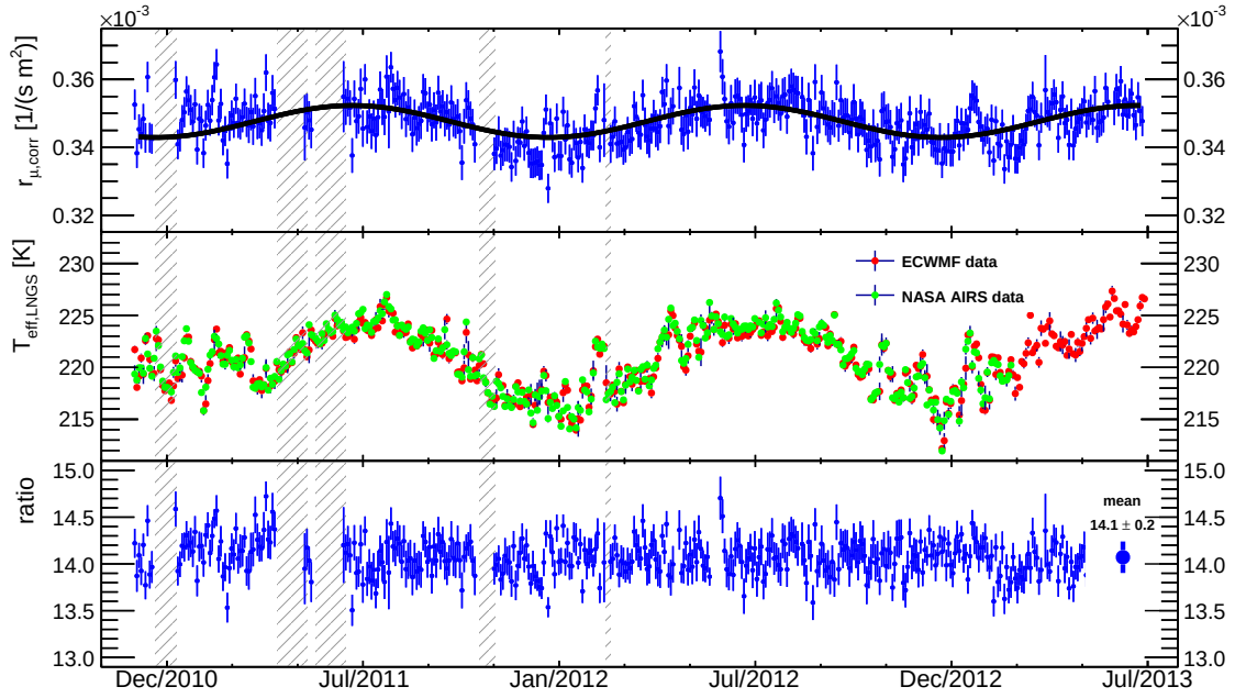
Figure 6.11: Top: the annual modulation of the rate of the muon flux. Middle: effective atmospheric temperature T_{\text{eff}} for the muon production. The data set of the ECWMF [ECW13] is shown in red, the set of the AIRS module on-board the NASA Aqua satellite [Par03] is shown in green. Bottom: ratio of the two.
