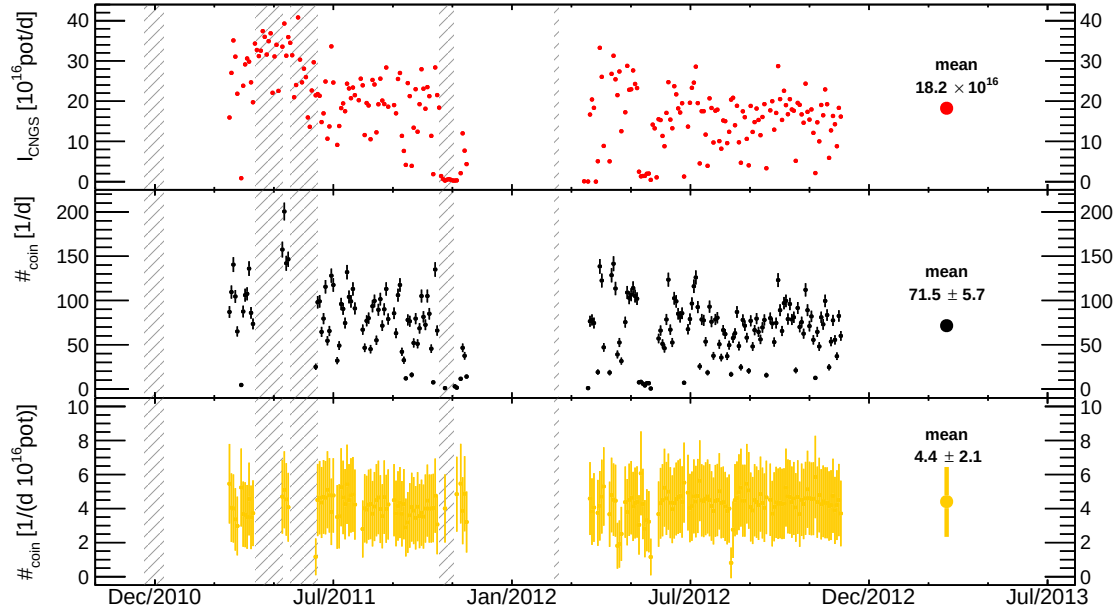
Figure 6.7: CNGS beam intensities and coincident events over time. The top panel shows the beam intensity measured at CERN. The medium panel shows the coincident events as defined by the main peak structure in Fig. 6.6. The bottom panel shows the ratio, which indicates that the number of coincident events is proportional to the beam intensity. The grey hatched areas mark pauses in the muon data-taking.
