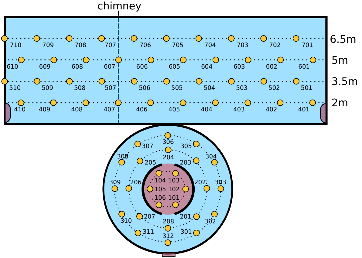
Figure 5.3: Distribution and naming scheme of the PMTs.
