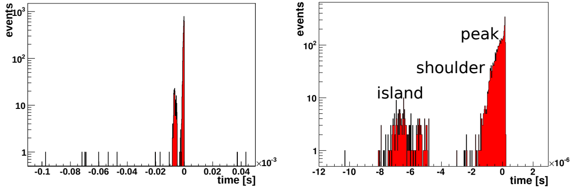
(a) 160 \mu\text{s} window equivalent to the germanium trace. Muon events in this time frame fulfil the condition isVetoIntime . (b) 15 \mu\text{s} window. Loosely equivalent to the contrast. Muon events in this time frame fulfil the condition isVetoIntime .
