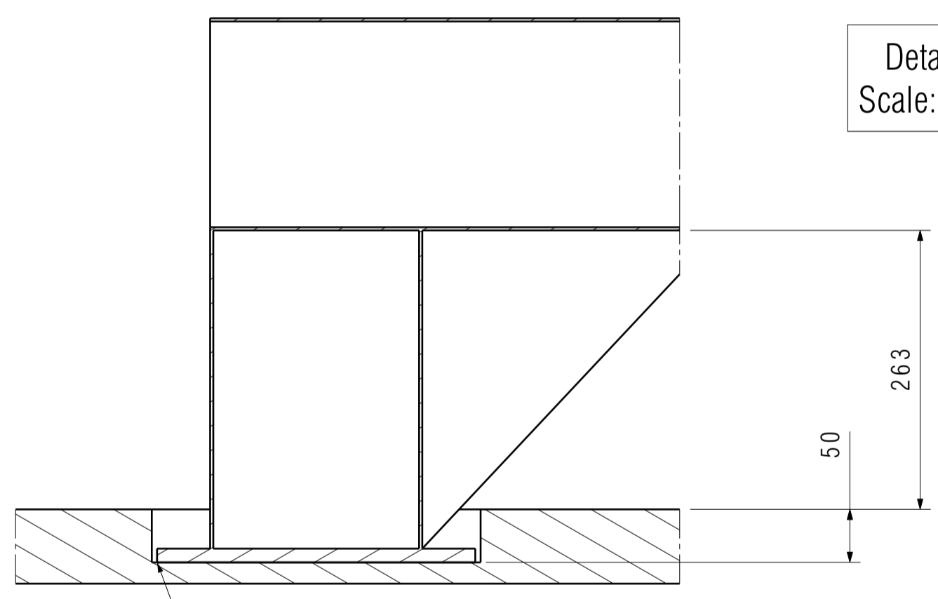
Section view D-D Scale: 1:5
