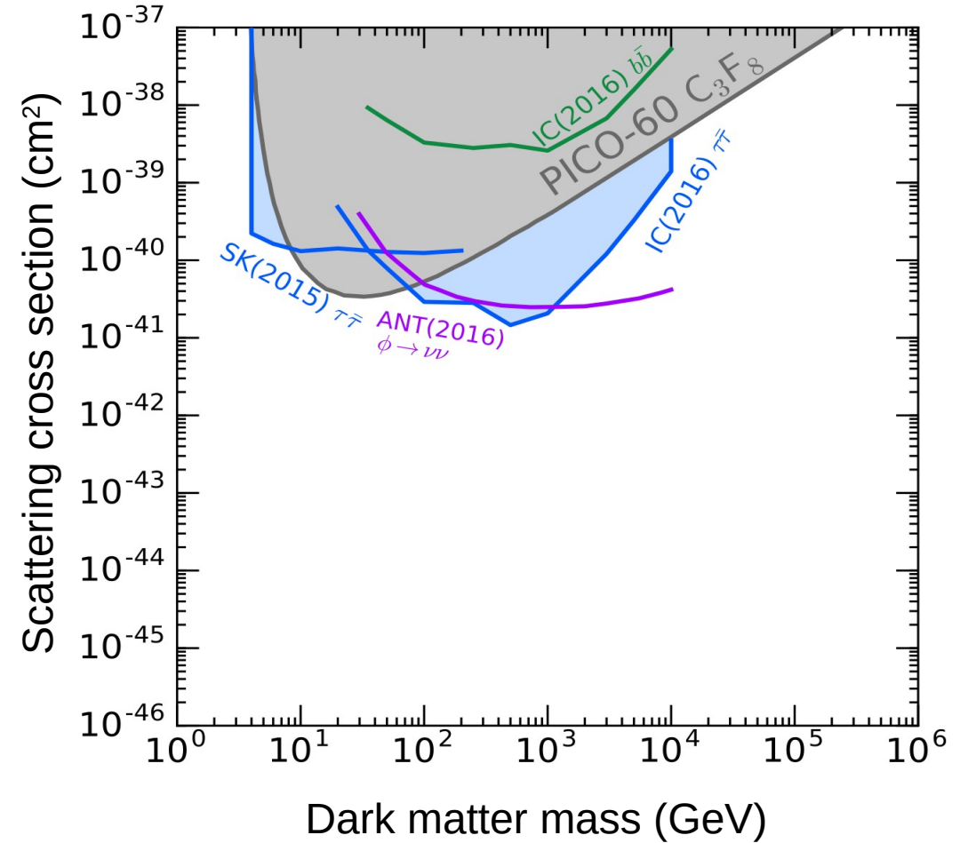
Limits from neutrinos, standard scenario
