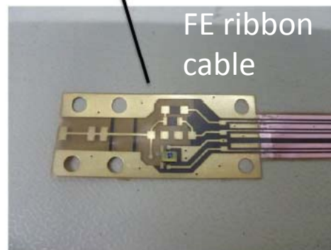
flex cables with JFET and feedback resistor/capacitor
