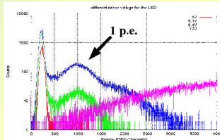
Light output of the system 1 for different supply voltages of the LED.
