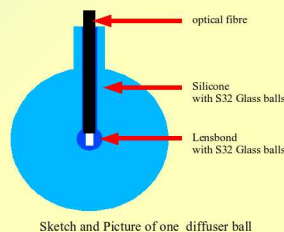
Sketch and Picture of one diffuser ball
