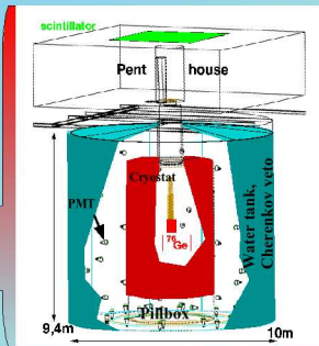
GERDA-geometry, with final PMT distribution, used for the Monte-Carlo-simulations, implemented in the MaGe framework.
