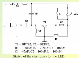
Sketch of the electronics for the LED.
