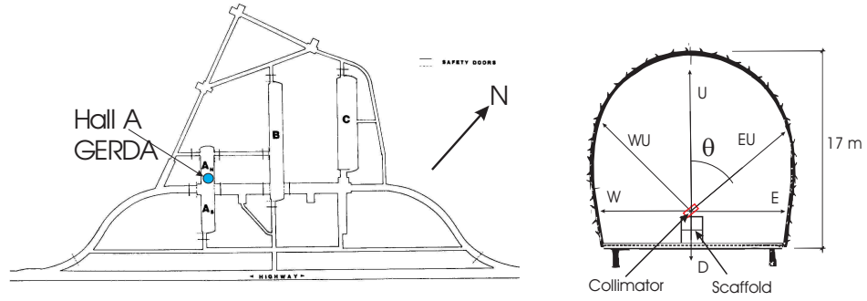
Figure 6.7: Left: floorplan of the LNGS underground laboratory. The location of GERDA in Hall A is indicated. Right: the detector for the \gamma -flux measurements was positioned on a scaffold \sim 2.5 m above the ground. The angular distribution of the \gamma -flux was measured with the collimator pointing into the indicated directions, and also to the north and to the south (direction assignments are: W-west, WU-West-Up, etc., \theta=0 in zenith).
