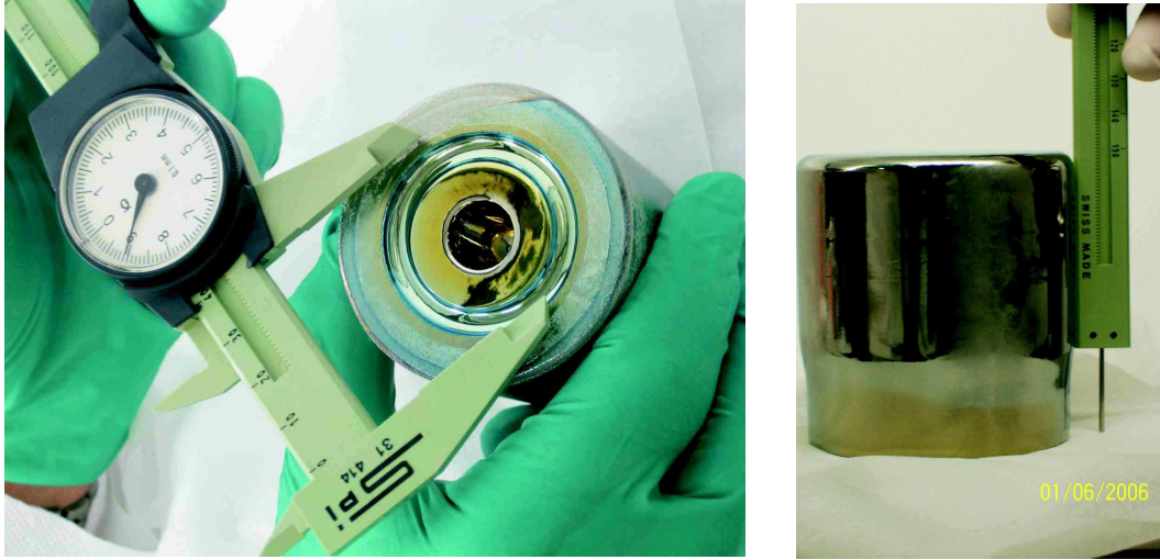
Figure 7.5: The enriched detectors ANG1 (left) and RG3 (right) after opening of the cryostats and detectors holders. Dimensions measurements were performed on the Class 10 clean bench in GDL at LNGS.
