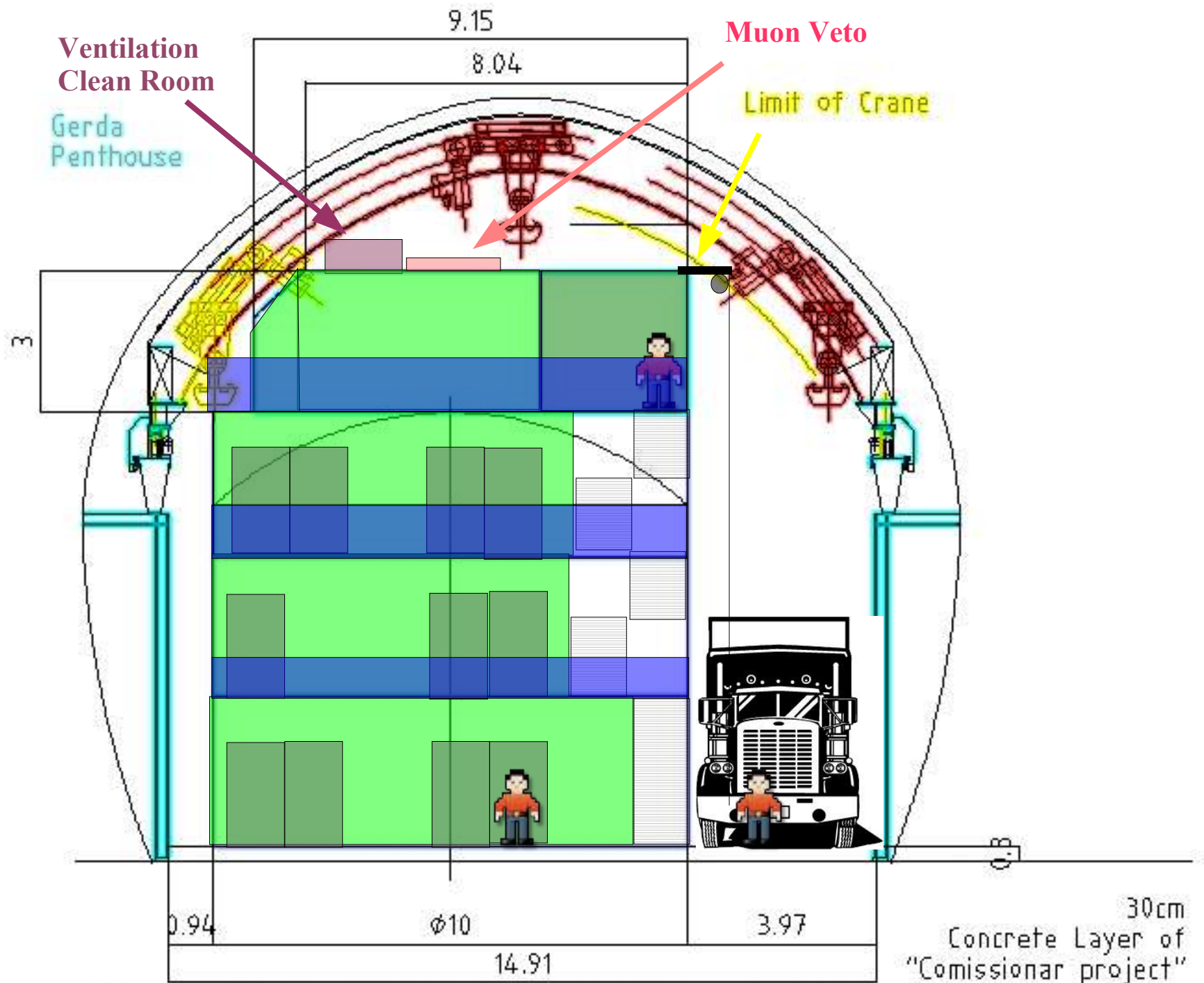
TRANSVERSAL CROSS SECTION HALL A FROM LVD TO GERDA
