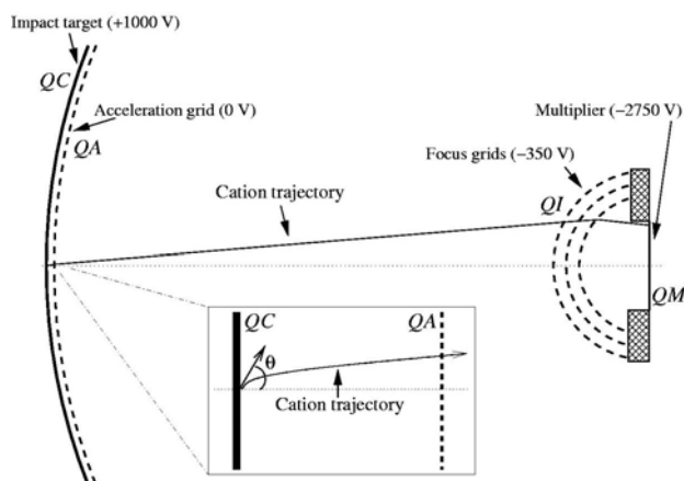
Figure 1. Schematic of the Chemical Analyser, showing the spherical section rhodium target (left) and the multiplier (right). Electrons detected on the target give a charge signal QC, and ion signals QA, QI and QM are obtained from ions impacting the accelerating mesh, the multiplier focus grids, and the multiplier respectively (QM being the actual spectrum signal). The initial ion emission angle is defined by \theta . The cation trajectory shows the case where an ion is 'just detected'.
