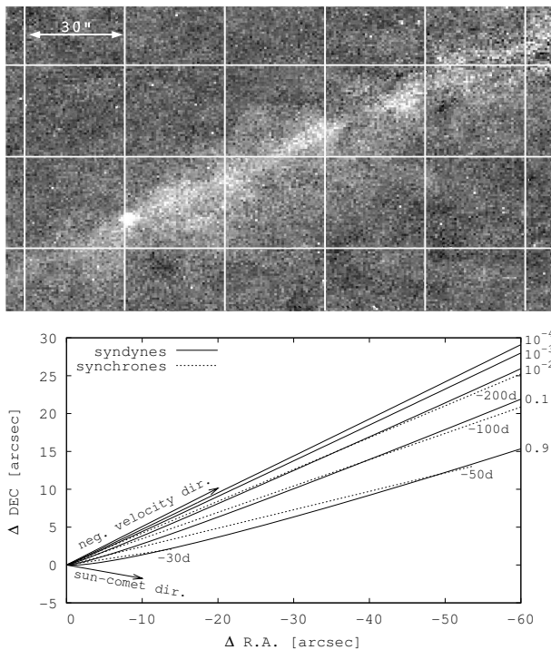
Figure 3. Top: Enlarged view of the nucleus and adjacent region in Fig. 1(a) before rotation. Bottom: A plot of synchronones and syndynes for 19 April 2004. Synchronones are the positions of particles of different \beta emitted at fixed times, labelled in the plot in days before observation. Syndynes show the positions of particles of given \beta (indicated at the right margin) released at varying dates. The negative orbital velocity vector of the comet corresponds to its projected orbit and trail axis. Syndynes of large and synchronones of old particles in the image converge towards this direction. The extended sun-comet vector points to where young, small grains of high \beta are expected to be found. In both images, north is up and east is left.
