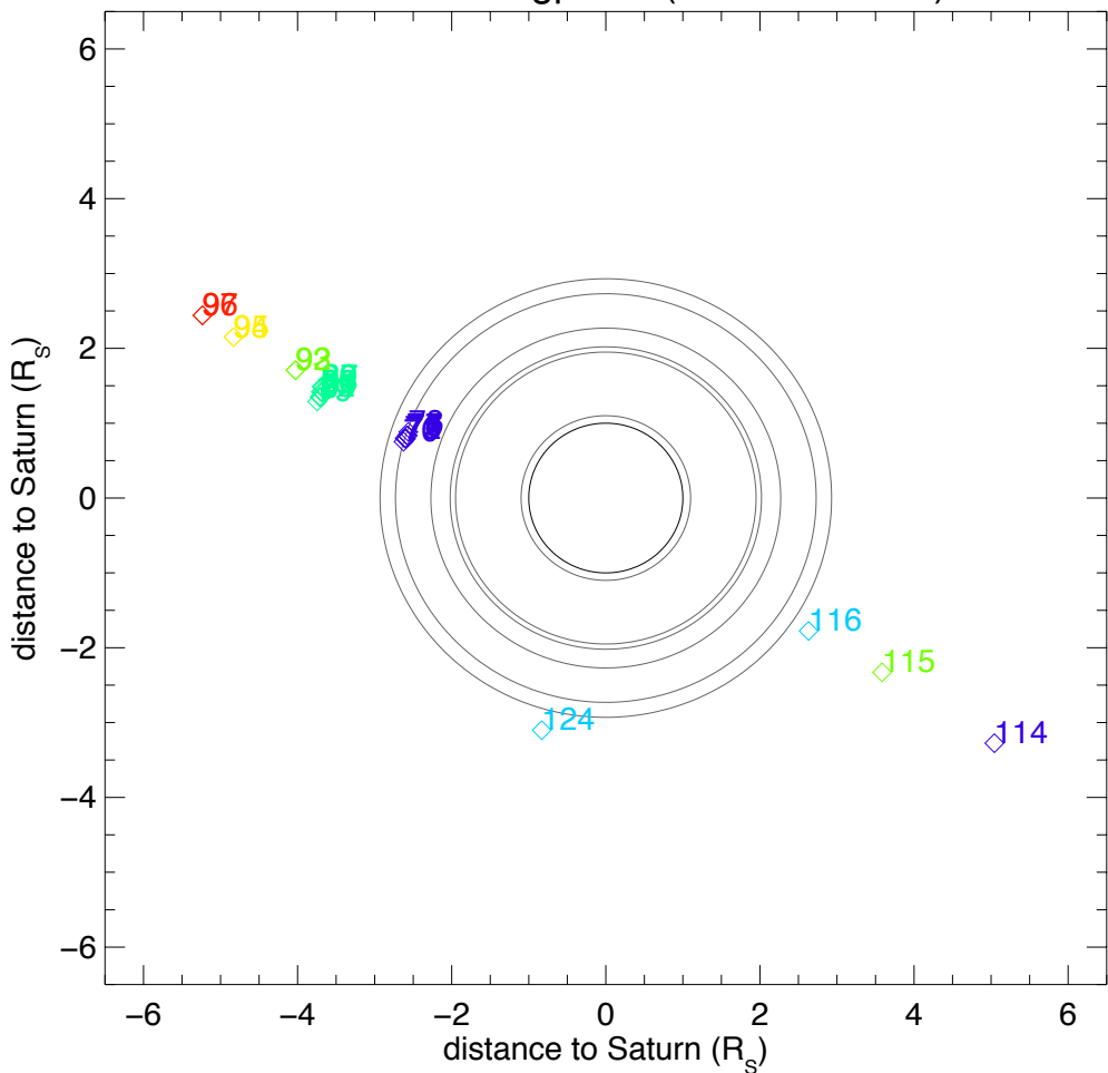
RPX within Ringplane (+x toward Sun)
