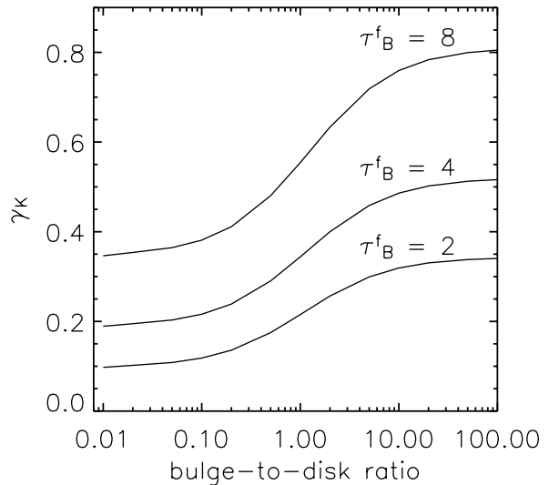
Fig. 8. The slope \gamma_K versus the intrinsic bulge-to-disk ratio, where \gamma_K is the slope of a linear fit to the low inclination part ( 1 - \cos i < 0.7 ) of the composite attenuation curve ( \Delta m vs. -\log(\cos i) ) in the K band. The calculations were performed for \tau_B^f = 8, 4, 2 .
