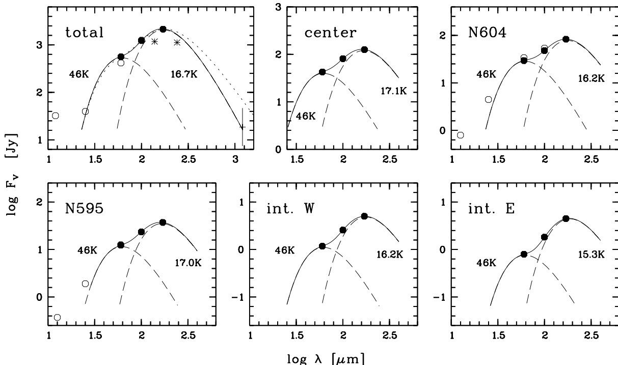
Fig. 3. Spectral energy distribution for total M 33 (top left), for the central area (top center), for two prominent H II regions (NGC 604, NGC 595), and for two areas in the interarm regime, W int. (offset 6' W, 5' S from the nucleus) and int. E (8' E from the nucleus). Dots are ISOPHOT data, circles stand for IRAS, asterisks for COBE/DIRBE data, and the plus with the large error bar at 1200 \mu\text{m} is derived from flux density ratios as estimated by Chini et al. 1986). Two-component blackbody fits for temperatures of T_{\text{warm}} = 46.0\text{ K} , T_{\text{cold}} \sim 16.5\text{ K} , respectively, and with emissivity \beta \propto \lambda^{-2} are overlaid as dashed and solid lines. For comparison, the dotted line shows a fit for \beta \propto \lambda^{-1} with T_{\text{warm}} = 52.0\text{ K} , T_{\text{cold}} = 19\text{ K} .
