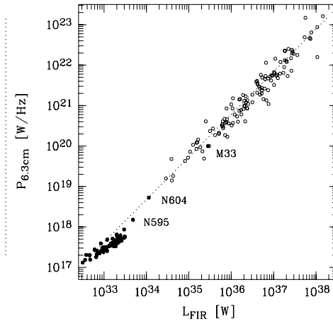
FIGURE 7. Plot of the monochromatic radio luminosity versus the FIR luminosities for M 33 (Hipelein et al. [42]) and its star-forming regions (filled circles) together with the data for the Effelsberg 100-m galaxy sample (Wunderlich et al. [99], open circle). The dotted line has a slope of 1.10 (Wunderlich & Klein [98]).
